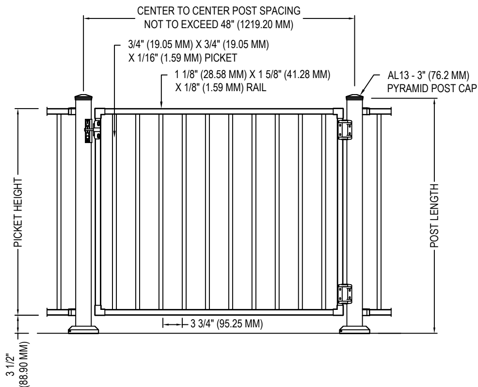
FRONT VIEW
